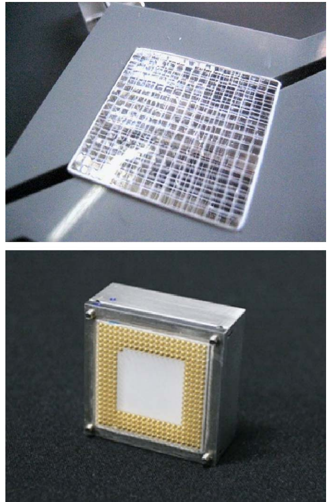
Fig. 4. (Upper) A picture of the 16 \times 16 LYSO matrix. (Lower) The TYP2 APD-array coupled with a LYSO matrix.
