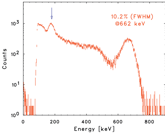
Fig. 5. An example of 662 keV gamma-ray spectrum obtained using the LYSO matrix coupled with the TYP1 APD-array.
