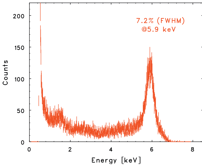
Fig. 3. An example of 5.9 keV X-ray spectrum measured with the TYP1 array.
