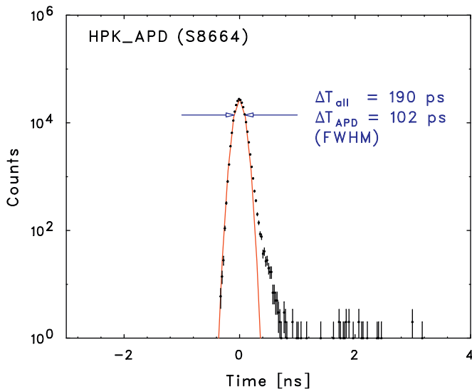
Fig. 6. Time response of the pixel APD S8664-30 measured with 16 keV X-rays.
